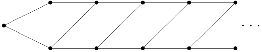
Figure 7: Bratteli diagram of the Sturmian tree S
