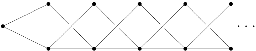
Figure 6: Bratteli diagram of the Fibonacci tree F
