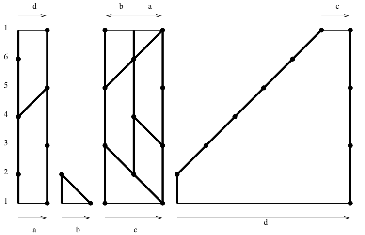
FIGURE 3. A simpler picture of the folded mapping torus with the unsubdivided cell structure. The six vertices v_1, \dots, v_6 are those at the heights 1, \dots, 6 as indicated.
