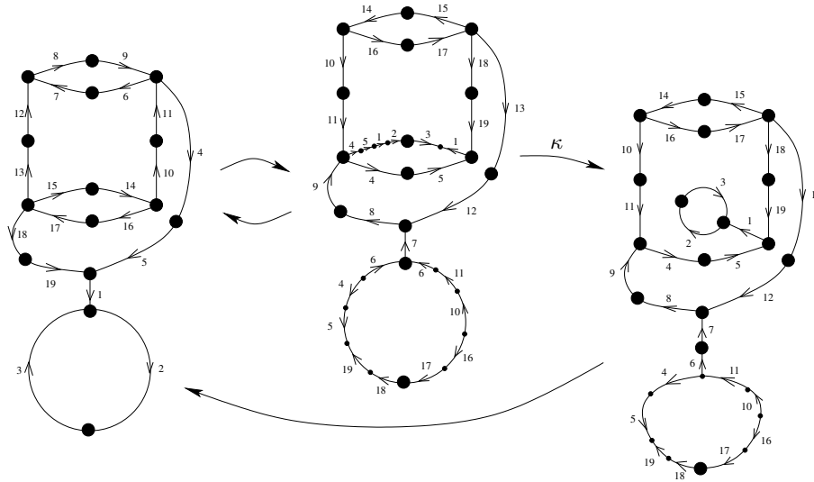
FIGURE 5. The first return map map f_1 : \Theta_1 \rightarrow \Theta_1 for the section \Theta_1 dual to [z_1] and the result of Stallings folds \kappa on the right.
