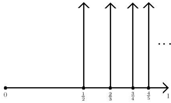
Example 2.16 Geodesically complete, not complete
